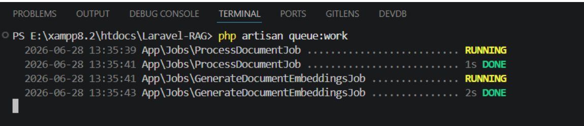
Figure 5: Background Job Processing Interface
